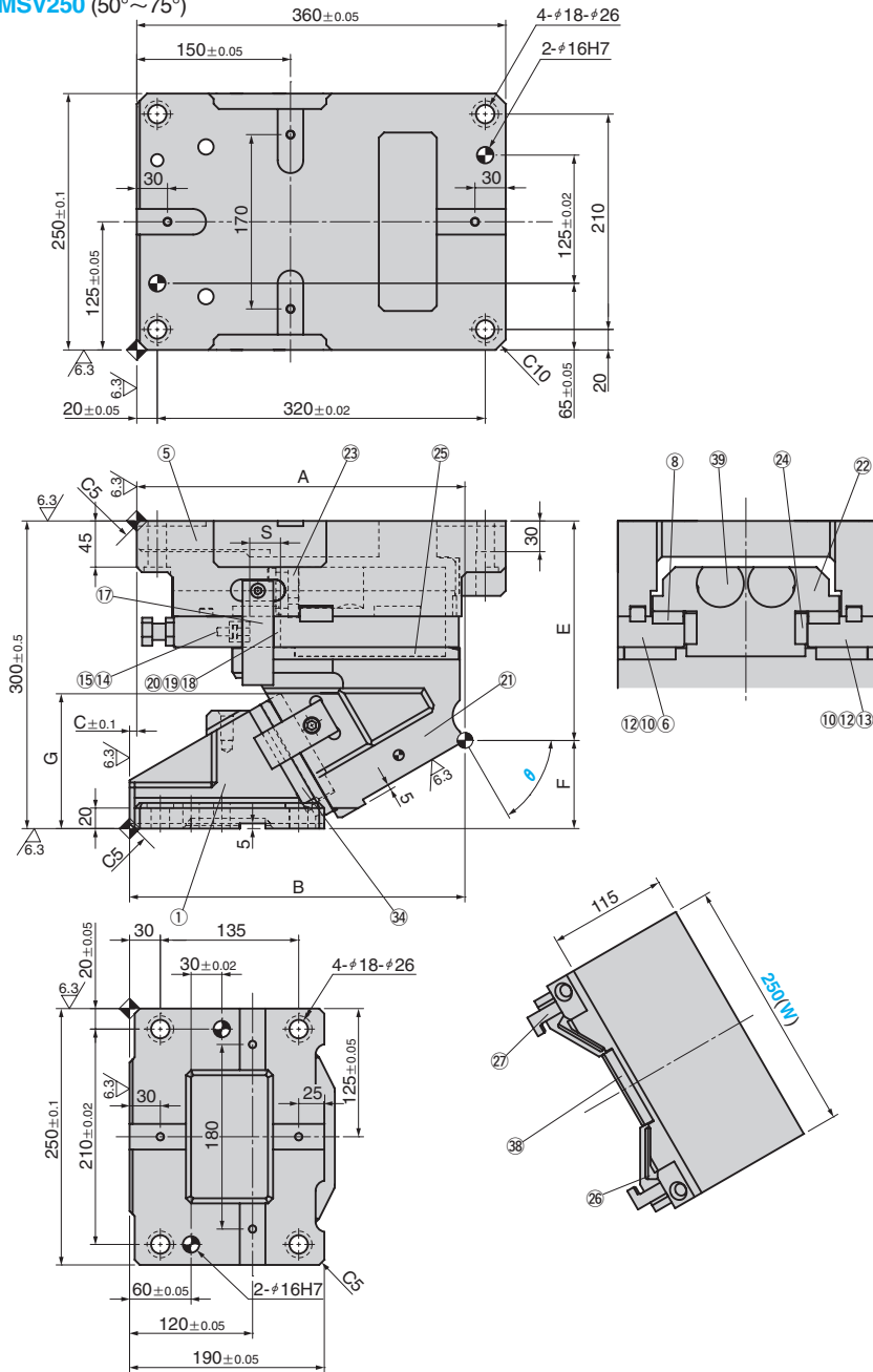
UCMSV250 (50°~75°)
