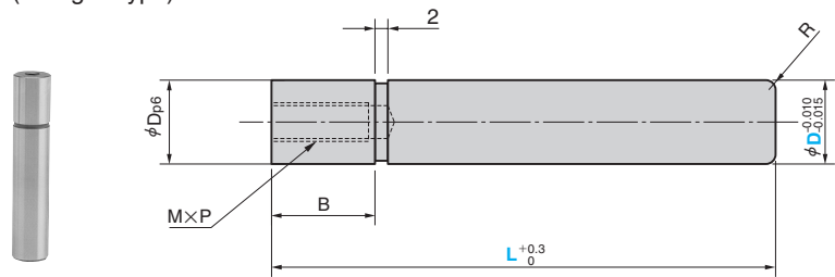
SUBGA (Straight Type)
