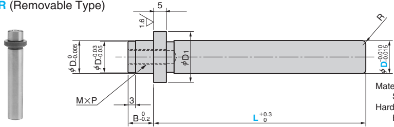
SUBGR (Removable Type)
