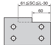
SC Specification Drawing
