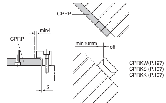
SC Specification Drawing
